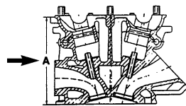
2 valve head
